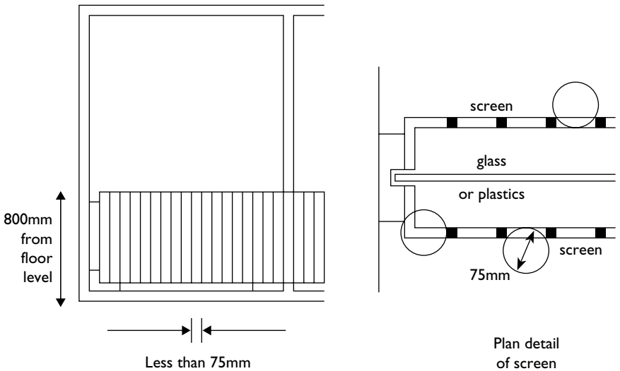
Figure 2 – Permanent screen protection
